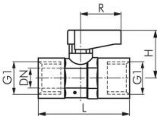
Version: Female - Female Thread
