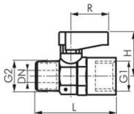
Version: Female - Male Thread
