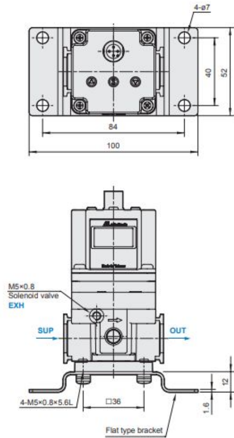
Flat type bracket
