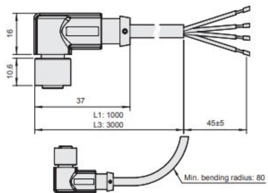
Angle cable connector
