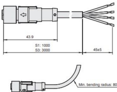
Straight cable connector
